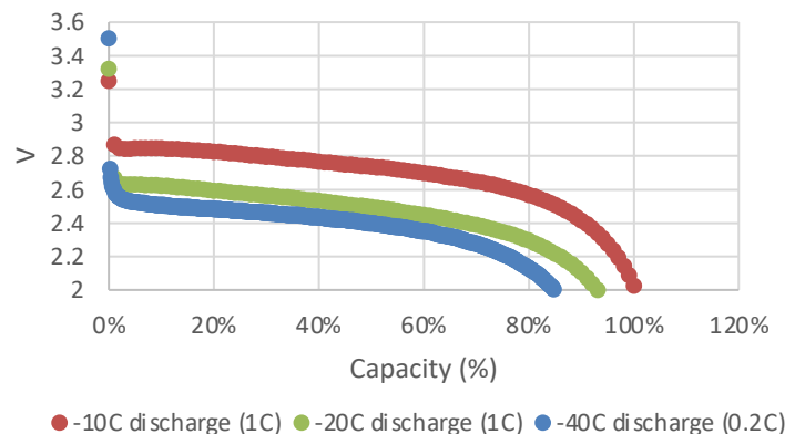
NVP-100 Low Temperature discharge test (2.0~3.6V)
