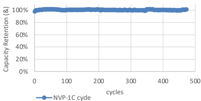
NVP-1C cycle 2.0~3.6V
